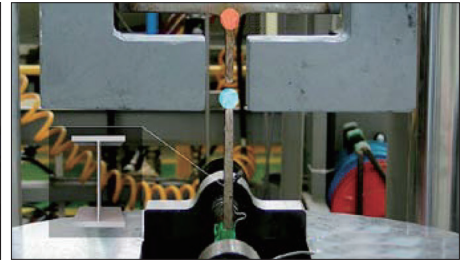
Welding joint tensile test
